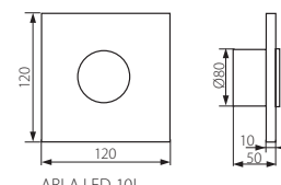
ARLA LED-10L
