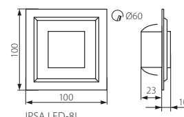
IPSA LED-8L
