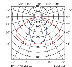
TEAR MTH-70-GR
