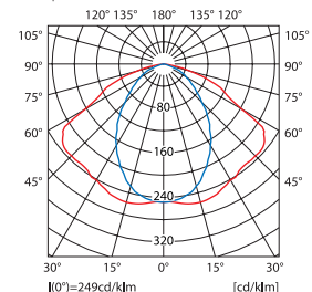
TEAR MTH-150-GR
