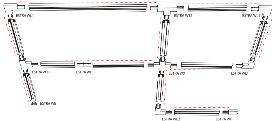
..... earth The way of assembly and power supply of the single phase track system ESTRA
